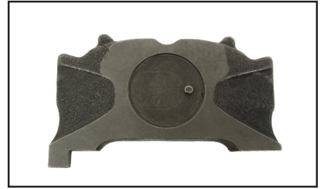
220394 Left Hand Pad Plate With Pin For 17.5" Wheels
