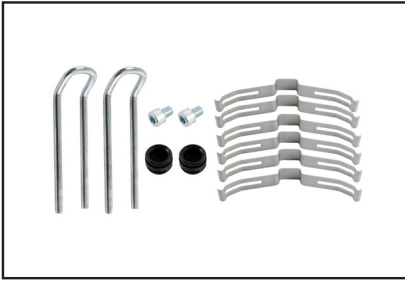
P67RK019AMultifit: Caliper Pad Retainer Kit Fits Caliper Type: WABCO Max 22
