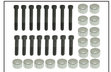
P67RK002EMultifit: yes Bolt & Bush Kit Fits Caliper Type: PAN17, PAN19, PAN22, 17.5"
